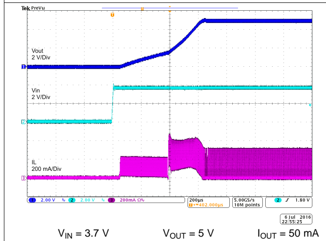
Figure 19. Startup by V_{IN}
