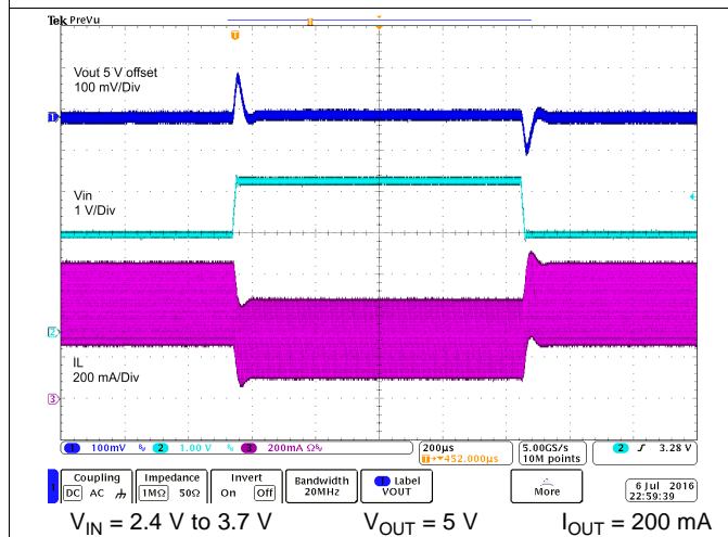
Figure 21. Line Transient
