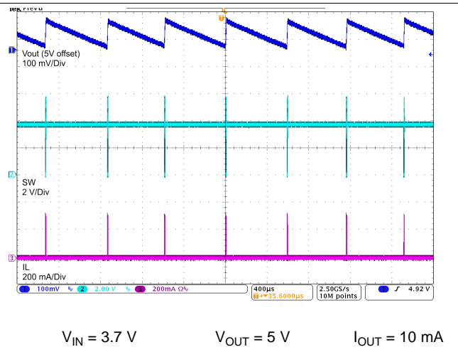
Figure 18. Switching Waveform at Light Load
