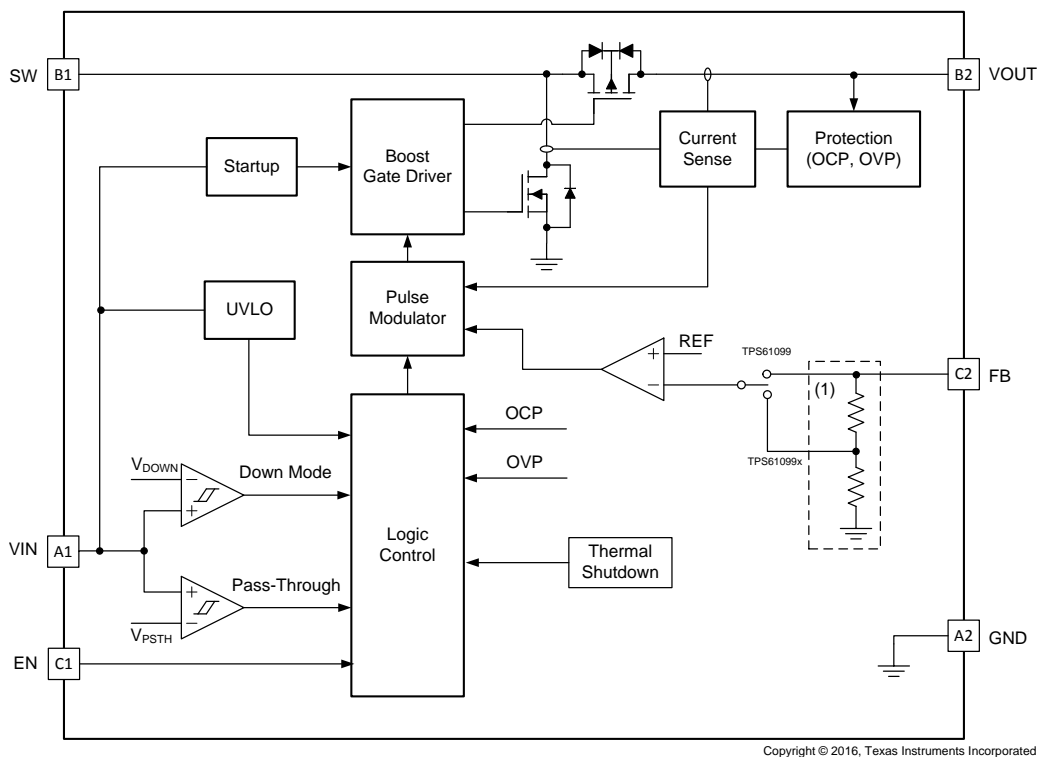
Figure 13. Functional Block Diagram
