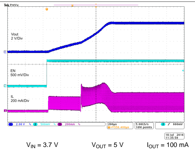
Figure 20. Startup by EN
