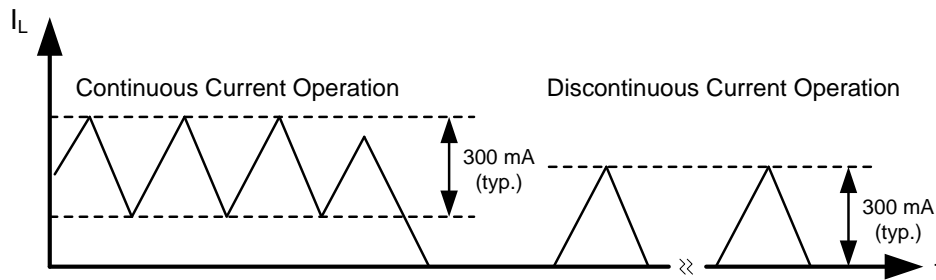
Figure 14. Hysteretic Current Operation
