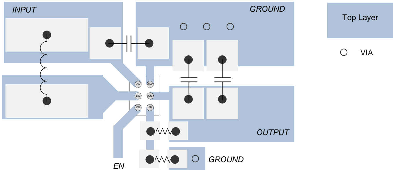
Figure 25. Layout
