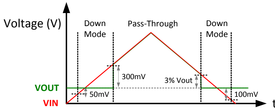
Figure 16. Down Mode and Pass-Through Operation
