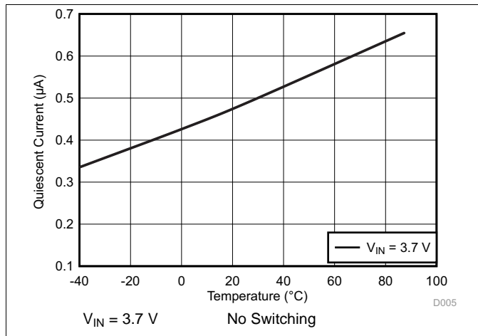
Figure 7. Quiescent Current into V_{\text{IN}} vs Temperature
