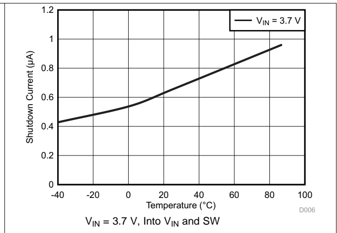
Figure 8. Shutdown Current vs Temperature
