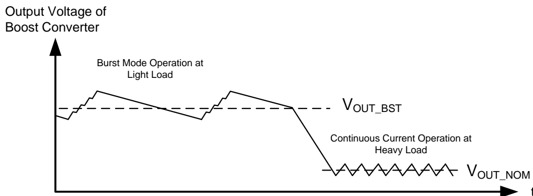
Figure 15. Burst Mode Operation
