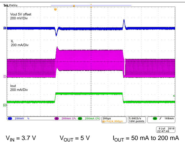
Figure 22. Load Transient
