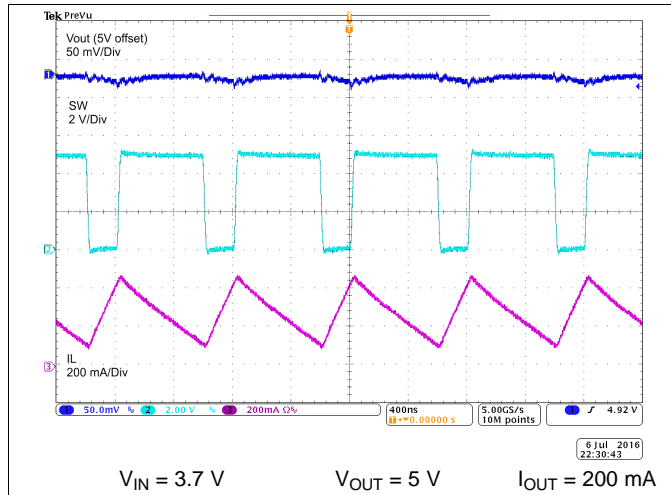
Figure 17. Switching Waveform at Heavy Load
