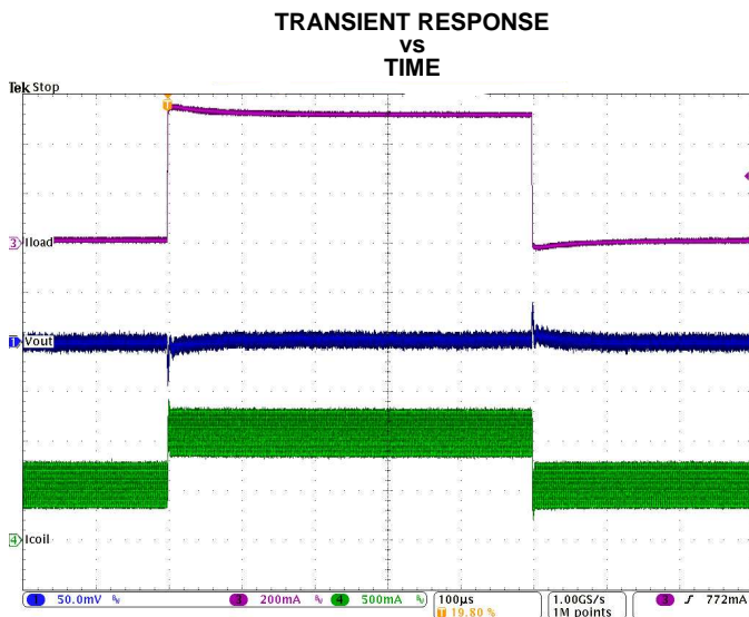
Figure 25. Load Transient Response in PWM mode (500mA to 1A)
