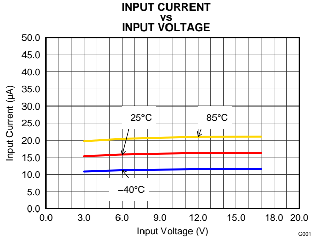
Figure 17. Quiescent Current
