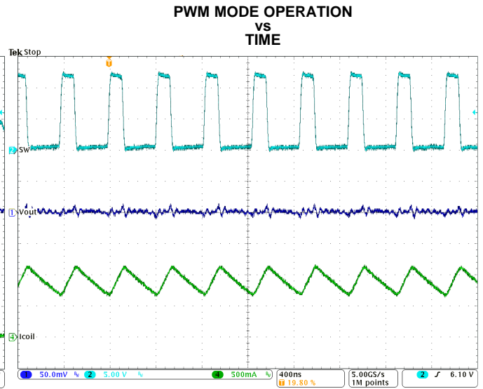
Figure 32. Typical Operation in PWM Mode (Iout=1A)
