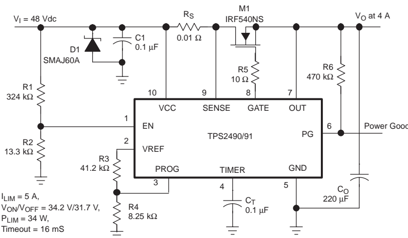
Figure 1. Typical Application and Corresponding SOA
