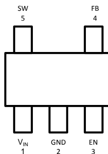
Figure 3. SOT-23-5 Package (Top View)
