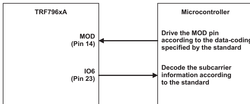
Figure 6-22. Control of RF Modulation Using MOD
