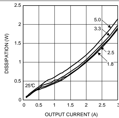
Figure 6. Dissipation 24-V Input at 25°C
