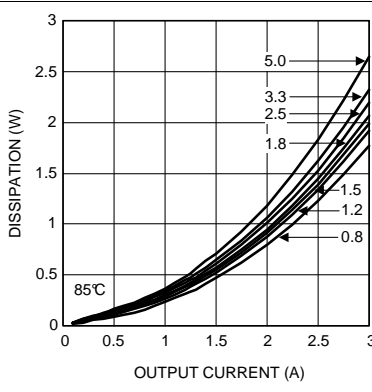
Figure 12. Dissipation 8-V Input at 85°C
