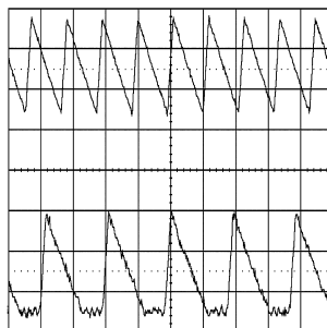
Figure 25. CCM and DCM Operating Modes V_{IN} = 24 \text{ V} , V_O = 3.3 \text{ V} , I_O = 3 \text{ A} /0.4 A 2 \mu\text{s}/\text{div}
