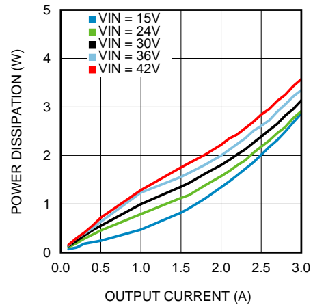
Figure 4. Power Dissipation V_{OUT} = 12\text{ V} , T_A = 25^\circ\text{C}
