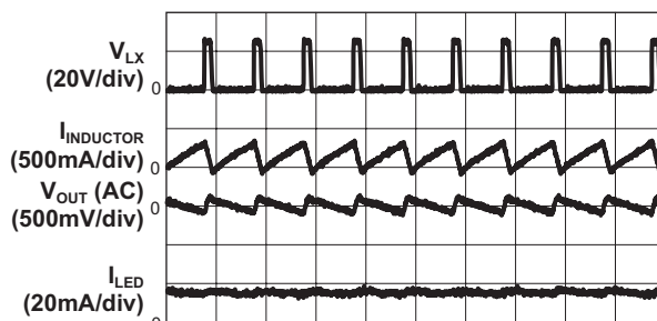
Operation Waveform with 50kHz PWM Control
