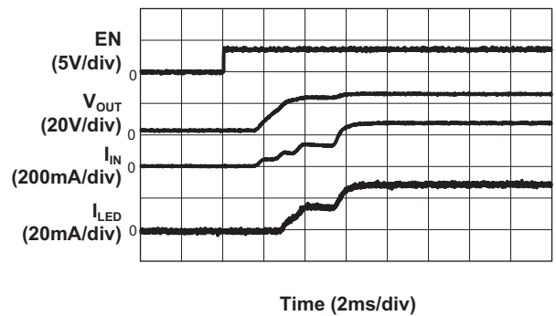
Startup Waveform
