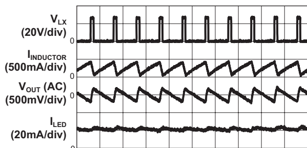
Operation Waveform
