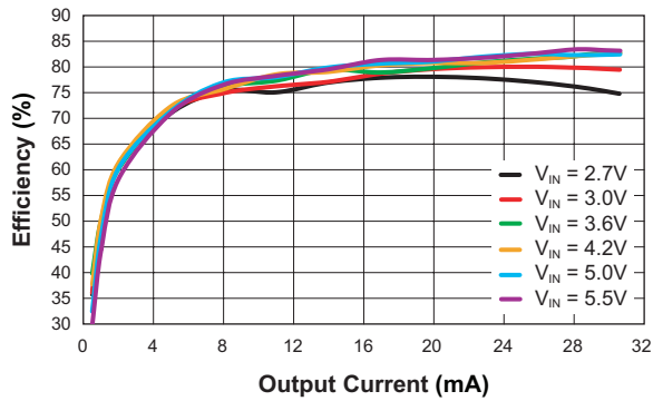
Efficiency vs. Output Current (R SET = 10KΩ, L = 10µH, 8 LEDs)
