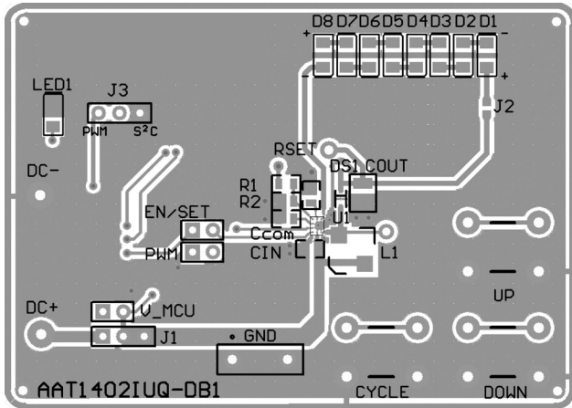
Figure 7: AAT1402 Evaluation Board Layout Top Layer.
