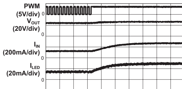
LED Current Transition by PWM
