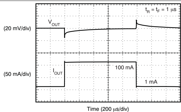
Figure 16. Load Transient 0
