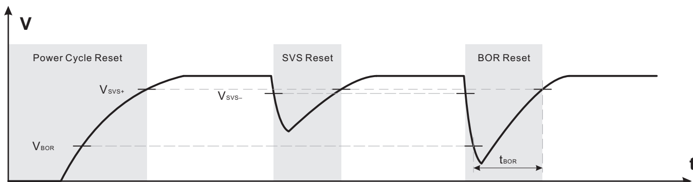
Figure 5-5. Power Cycle, SVS, and BOR Reset Conditions
