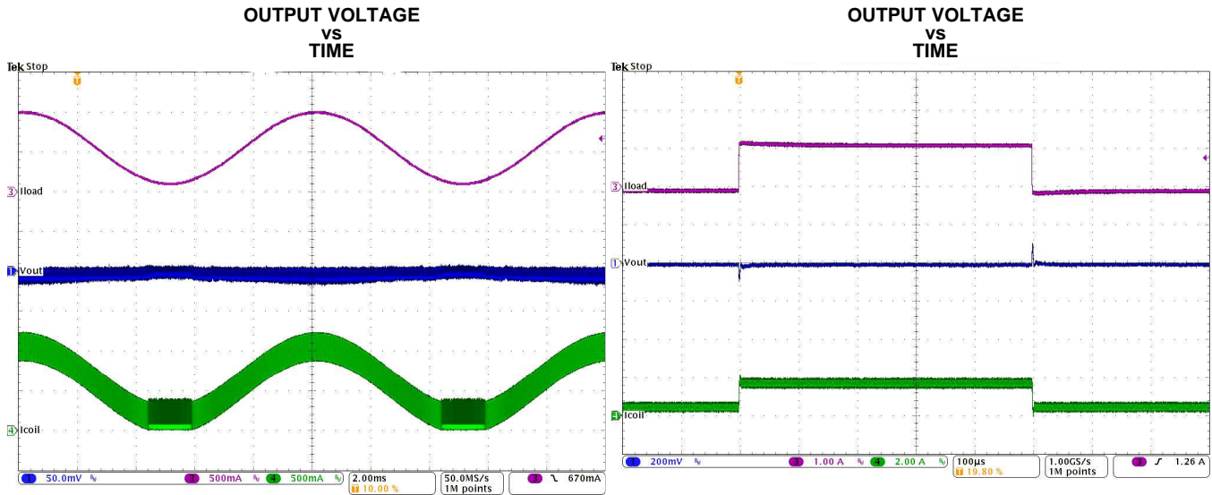
Figure 29. PWM-PSM-Transition ( V_{IN}=12\text{ V} , V_{OUT} = 3.3\text{ V} With 50 mV/div)
