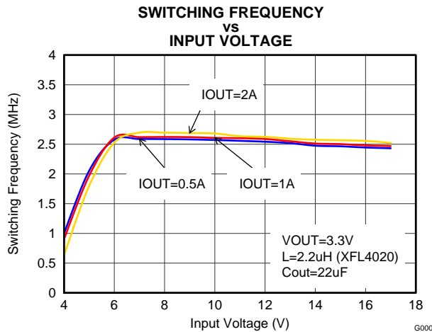
Figure 19. Switching Frequency
