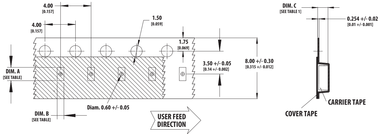
Figure 8. Tape Dimensions
